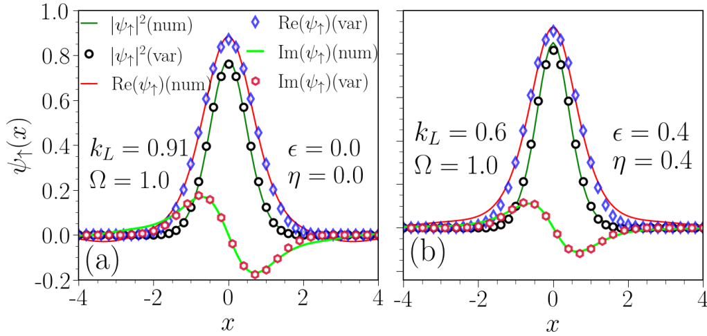
Figure 4.11: Ground state density profile obtained using numerical (with lines) and variational scheme (with markers) for (a) k_L = 0.91 , \epsilon(= \eta) = 0 , and (b) k_L = 0.6 , \epsilon(= \eta) = 0.4 . The real and imaginary parts of the spin-up condensate wavefunction obtained from the numerical simulation and variational approach agree well.
