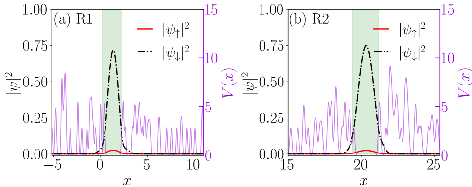
Figure 5.11: Condensate density at \Omega = 0.1 , U_0 = 0.5 . The interaction and SO coupling parameters are g_{\uparrow\uparrow} = 0.1 , g_{\downarrow\downarrow} = 0.05 , g_{\uparrow\downarrow} = 1.0 , and k_L = 0 . The random potential profile is shown with light violet lines along the right side axis. The shaded region is drawn to show the void of the potential.
