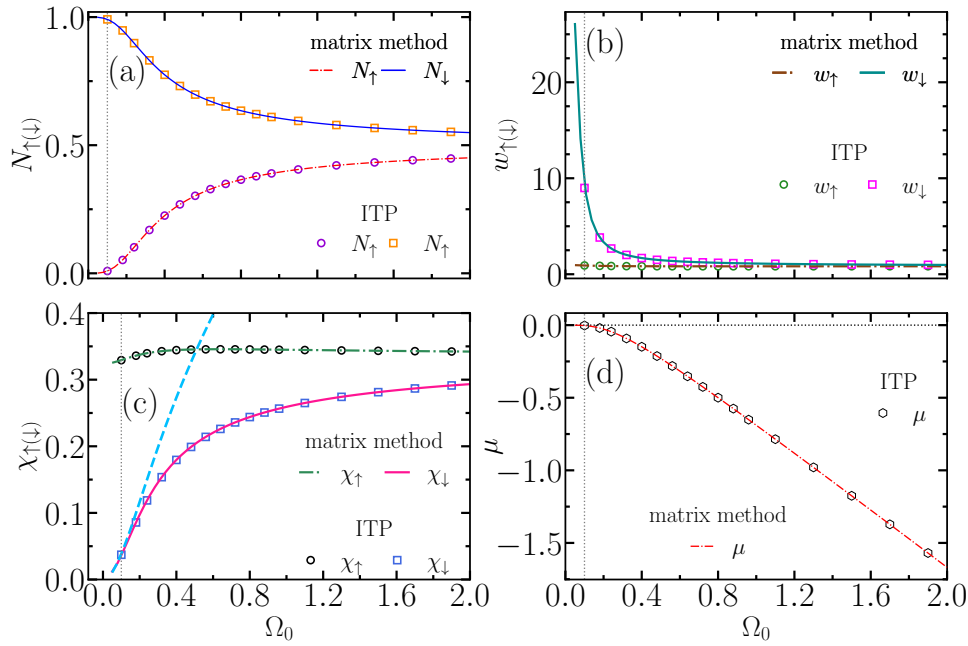
Figure 6.5: (a) Variation of population as a function of Rabi coupling \Omega_0 for V = V_\uparrow(x) = x^2/2 . (b) Width w_{\uparrow(\downarrow)} , (c) IPR \chi_{\uparrow(\downarrow)} , and (d) the chemical potential as a function of \Omega_0 at g = 0 . The increasing IPR indicates that the condensate of spin-down component tends to localize due to the interaction with spin-up one. In panel (c), the dashed cyan line is drawn to show the comparison with \chi_\downarrow = \sqrt{|\mu|/2} corresponding to \psi_\downarrow in Eq. (6.16).
