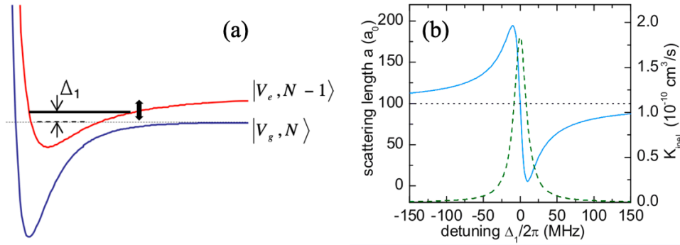
Figure 1.7: (a) Schematic diagram of optical coupling between collisional and molecular states. The excited potential |V_e, N-1\rangle is separated from the ground state potential |V_g, N\rangle by laser detuning \Delta_1 . Here, N is the number of photons in the light field. (b) Scattering length a (cyan solid line), and inelastic collision rate K_{\text{inel}} (green dashed line), which causes atomic loss as a function of laser detuning \Delta_1 obtained for a condensate of ^{87}\text{Rb} atoms. This figure is adapted from Ref. [75, 79].
