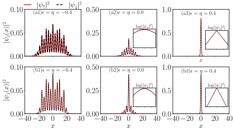
Figure 4.1: Density profile of |\psi_\uparrow|^2 (red line) and |\psi_\downarrow|^2 (dashed black line) components for different inhomogeneity parameter \epsilon = \eta = -0.4 (a1,b1), \epsilon = \eta = 0 (a2,b2), and \epsilon = \eta = 0.4 (a3,b3) at k_L = 0 , \Omega = 0.0 (upper panel) and k_L = 0.6 , \Omega = 1 (lower panel). Insets in [(a2, a3, b2, b3)] show the spatial variation of density profile in semilog scale that explicitly displays the exponential tail of the localized condensate in (a3) and (b3).
