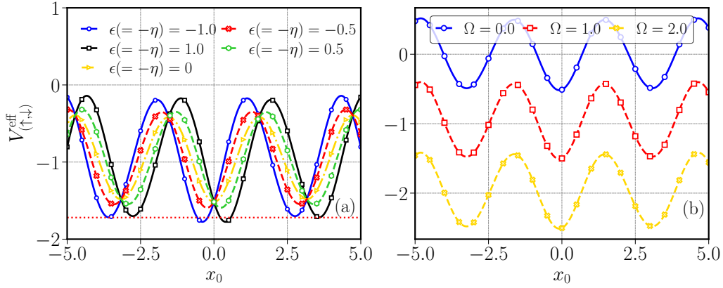
Figure 4.17: (a) Variation of effective potential ( V_{(1,2)}^{eff} ) as obtained in Eq. 4.15 of spin-components with x_0 for different inhomogeneous interaction parameters \epsilon(= -\eta) when the phase difference between the spatial inhomogeneity and potential considered is \pi/2 . For \epsilon = \eta = 0 , the potential is peaked at x_0 = 0 , which is the delocalized state. However, for |\epsilon(-\eta)| = 0.5 and 1, the central minima depth increases compared to those for zero inhomogeneity, indicating the localization state. (b) Variation of effective potential with x_0 for different \Omega with k_L = 0.6 , \epsilon = \eta = 0 . As the value of \Omega increases, the depth of the central potential also increases, implying that the Rabi coupling contributes towards the localization of the condensate.
