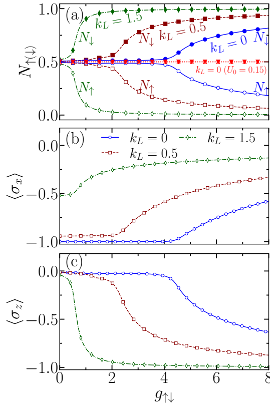
Figure 5.12: (a) Variation of populations with inter-species interaction g_{↑↓} by keeping intra-species interactions at g_{↑↑} = 0.1, g_{↓↓} = 0.5g_{↑↑} , and the coupling parameters are k_L = 0 (blue circle marked solid line), k_L = 0.5 (brown square marked dashed line), and k_L = 1.5 (green diamond marked dash-dotted line) at \Omega = 0.5 . Since g_{↑↑} > g_{↓↓} , owing to repulsion, we obtain N_{↑} < N_{↓} . Here, we also show the populations for U_0 = 0.15, k_L = 0 (red triangles with dotted line) in order to compare it with N_{↑(↓)} at U_0 = 0.5 (blue solid line). Variations of \langle \sigma_x \rangle and \langle \sigma_z \rangle as a function of inter-species interaction g_{↑↓} for k_L = 0 (blue solid line), 0.5 (brown dashed line), and 1.5 (green dash-dotted line) at U_0 = 0.5 are shown in panels (b) and (c), respectively.
