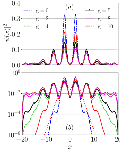
Figure 3.2: Variation of density with different nonlinearity for \lambda_1 = 10 , \lambda_2/\lambda_1 = 0.86 , s_1 = 3 , and s_2/s_1 = 1.0 in the (a) linear and (b) semilog scale. The wave function gets localized near x = 0 for g = 0 . As we increase the nonlinearity, it results in the spread of the wave function. In the localized states ( g = 0, 2, 4 ), the condensate density exhibits an exponential tail. For g \gtrsim 5 , the condensate gets spanned in the whole box, exhibiting a delocalized nature. In (b), the dotted red line represents the double exponential fit to the condensate ground state for g = 0 .
