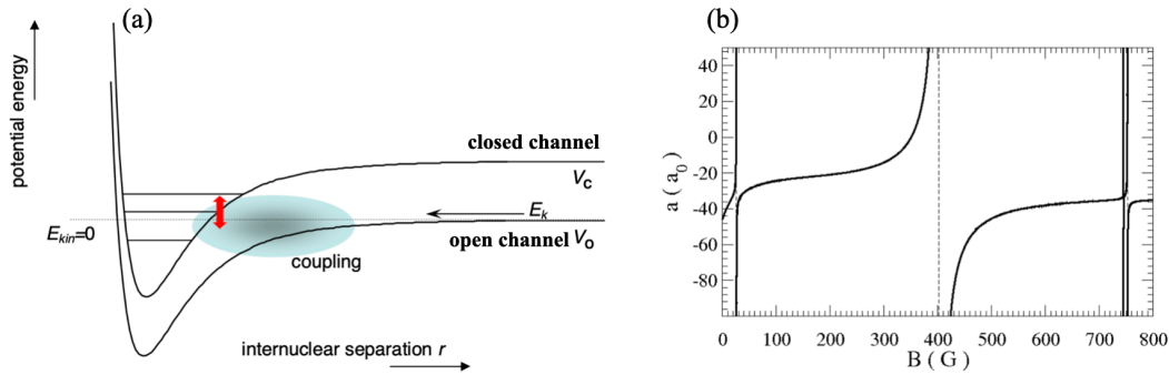
Figure 1.6: (a) Schematic diagram of the Feshbach resonance technique used in atomic collisions. The scattering state associated with the open channel V_o is coupled to the closed channel V_c of another atom. The coupling between these channels modifies the scattering potential and scattering phases, which can be controlled using an external magnetic field. (b) variation of scattering length with external magnetic field for ^{39}\text{K} atomic collisions of hyperfine states. The resonance condition is depicted by the vertical dashed lines. Figure is taken from [75, 35].
