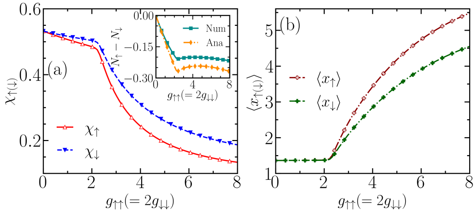
Figure 5.19: (a) Variation of the IPRs \chi_{\uparrow(\downarrow)} as a function of the intra-species interaction g_{\uparrow\uparrow}(= 2g_{\downarrow\downarrow}) for disorder strength U_0 = 0.5 . With the increase in g_{\uparrow\uparrow} , the IPR in both components decreases, resembling the broadening of the condensate irrespective of disorder strength U_0 . Other parameters are the same as Fig. 5.16. (b) The center of mass position for the up (red line) and down component (dashed blue line) as a function of the intra-species interaction g_{\uparrow\uparrow} .
