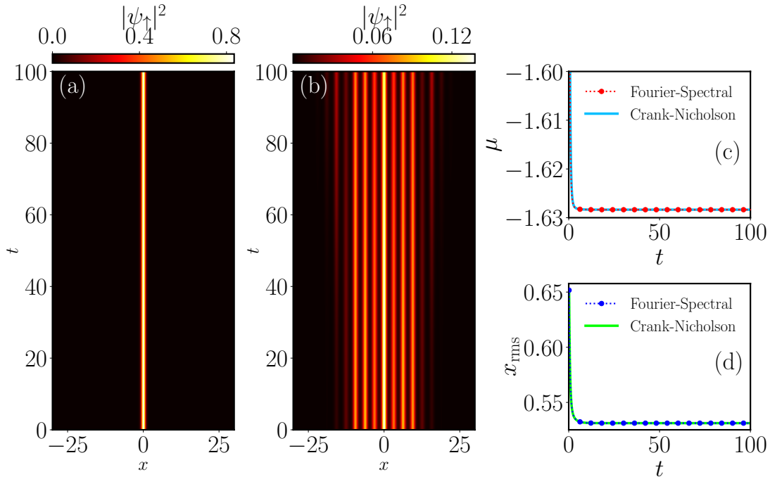
Figure 2.2: Spatio-temporal evolution of (a) localized and (b) delocalized condensate at k_L = 1.0 , \Omega = 1 , and k_L = 0.6 , \Omega = 1 , respectively. The temporal evolution of (c) chemical potential ( \mu ) and (d) rms size ( x_{\text{rms}} ) of the localized condensate. The temporal evolution shows the convergence of the localized ground state.
