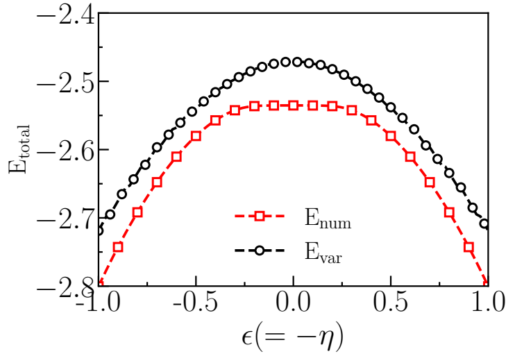
Figure 4.15: Variation of numerical ( E_{\text{num}} ) and variational ( E_{\text{var}} ) total energy with inhomogeneity \epsilon(= -\eta) with k_L = 0.6 , and \Omega = 1.0 . Tuning the inhomogeneity leads to a monotonic decrease in the total energy in the localized regions, that is -1 \lesssim \epsilon(= -\eta) \lesssim -0.3 or 0.3 \lesssim \epsilon(= -\eta) \lesssim 1.0 whereas, in the delocalized region -0.3 \lesssim |\epsilon(= -\eta)| \lesssim 0.3 , the total energy remains almost constant at E_{\text{num}} \sim -2.56 . In both cases, energy follow a symmetric nature in either side of delocalization regions.
